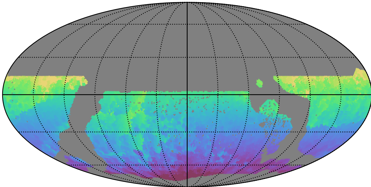
ddf_acor_sf10_lsf40_lsr10_v3.4_10yrs WFD all bands: Min HA
