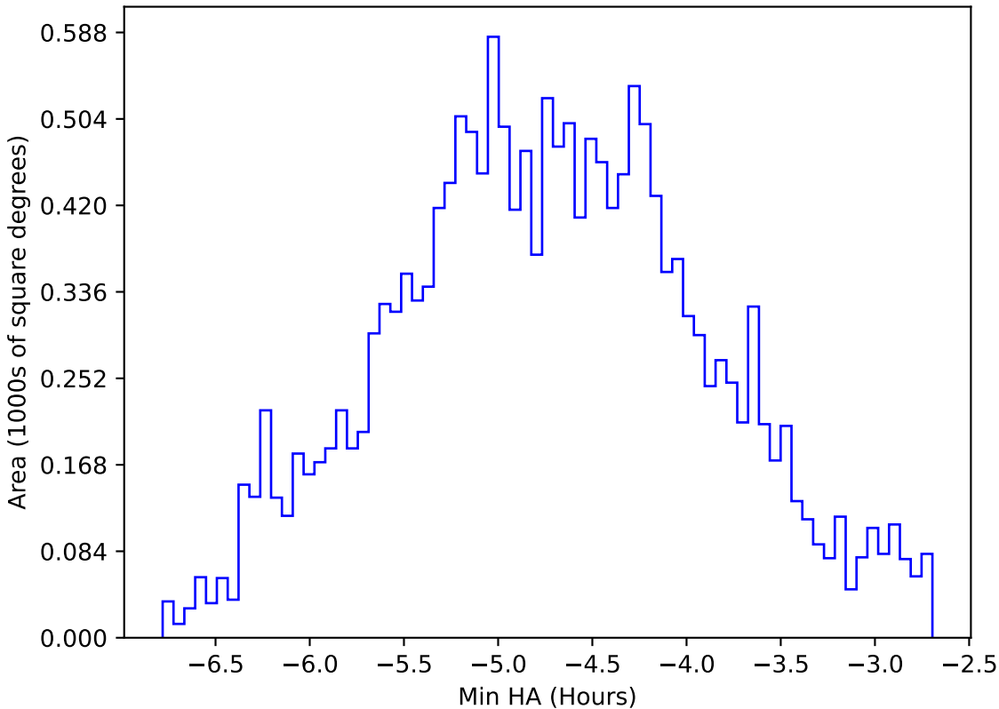
ddf_acor_sf10_lsf40_lsr10_v3.4_10yrs WFD all bands: Min HA
