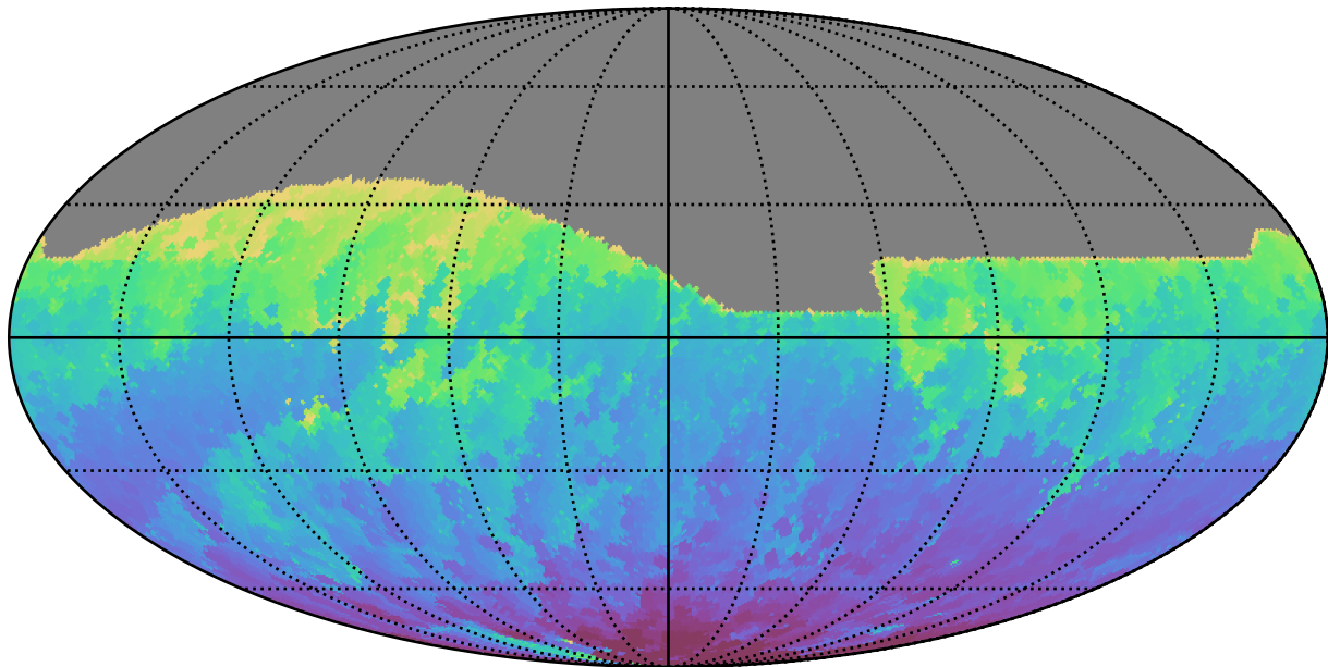
ddf_acor_sf10_lsf40_lsr10_v3.4_10yrs All sky z band: Min HA
