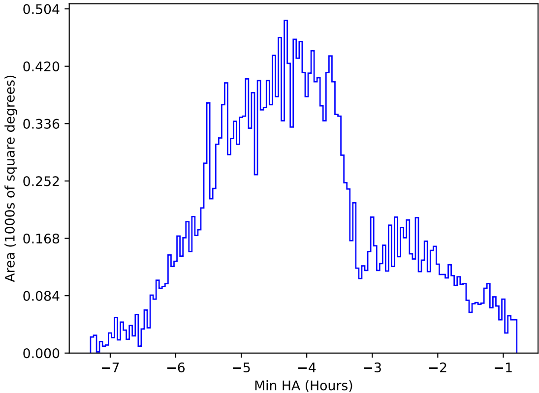
ddf_acor_sf10_lsf40_lsr10_v3.4_10yrs All sky z band: Min HA
