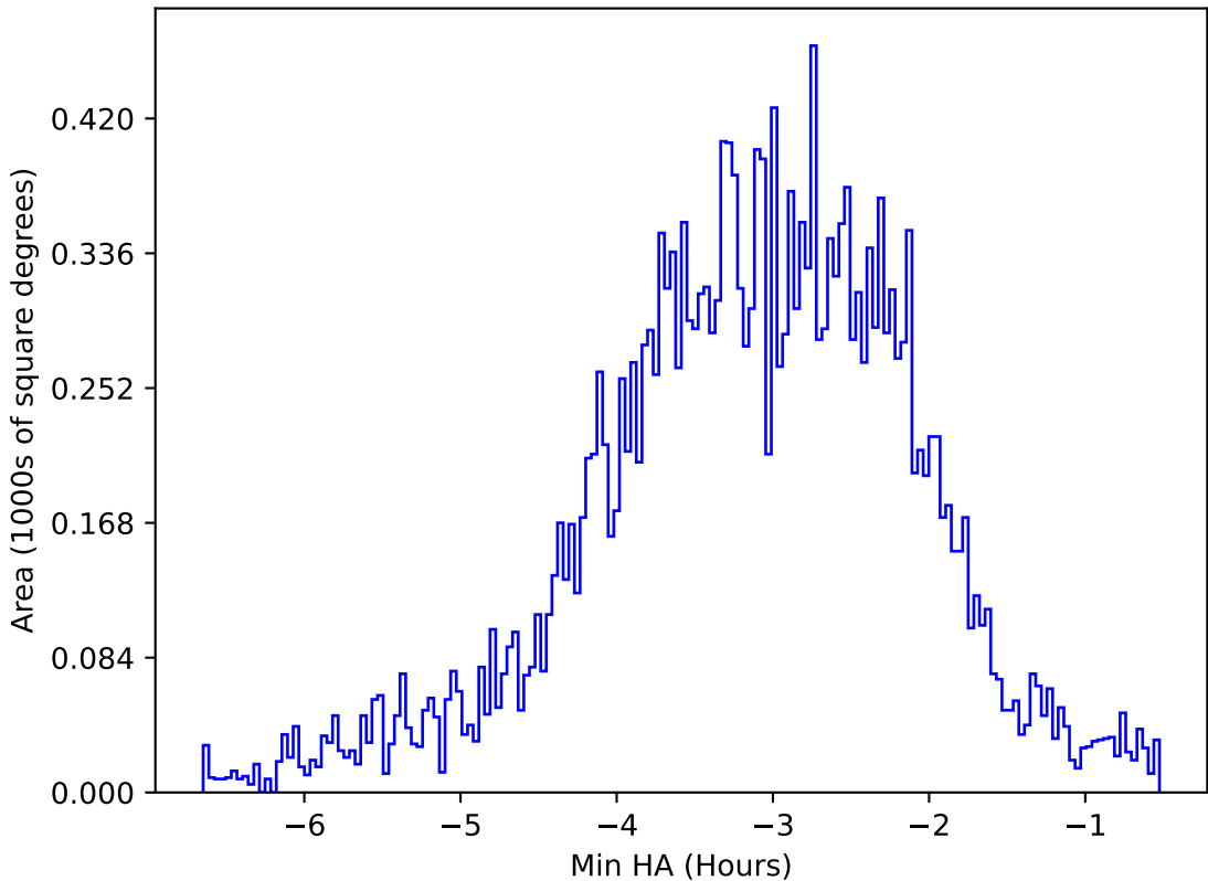
ddf_acor_sf10_ls40_lsr10_v3.4_10yrs All sky u band: Min HA
