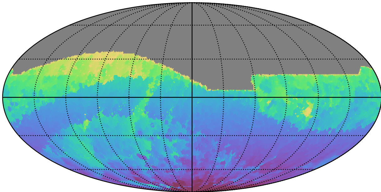
ddf_acor_sf10_lsf40_lsr10_v3.4_10yrs All sky r band: Min HA
