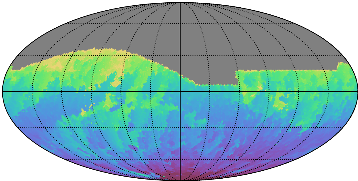
ddf_acor_sf10_lsf40_lsr10_v3.4_10yrs All sky i band: Min HA
