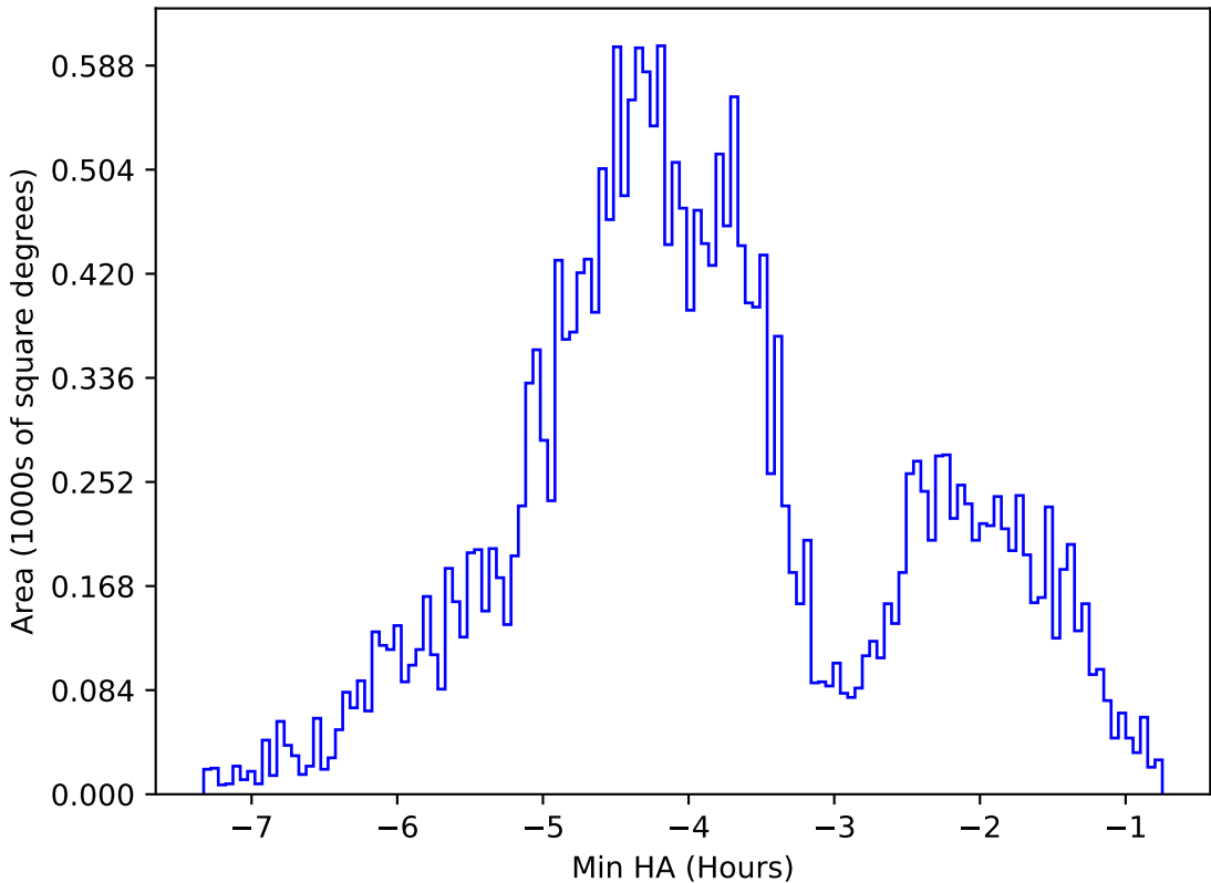
ddf_acor_sf10_lsf40_lsr10_v3.4_10yrs All sky g band: Min HA
