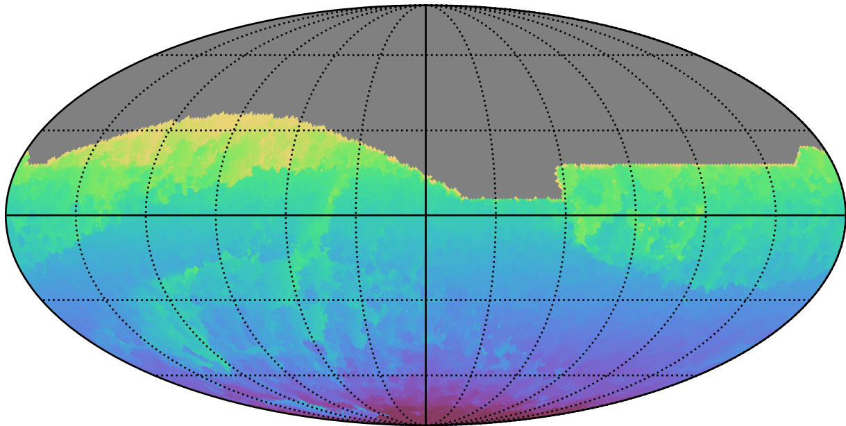
ddf_acor_sf10_lsf40_lsr10_v3.4_10yrs All sky all bands: Min HA
