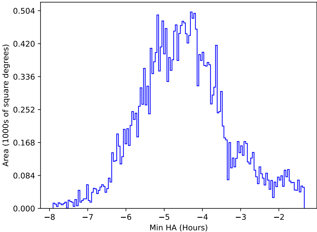
ddf_acor_sf10_lsf40_lsr10_v3.4_10yrs All sky all bands: Min HA
