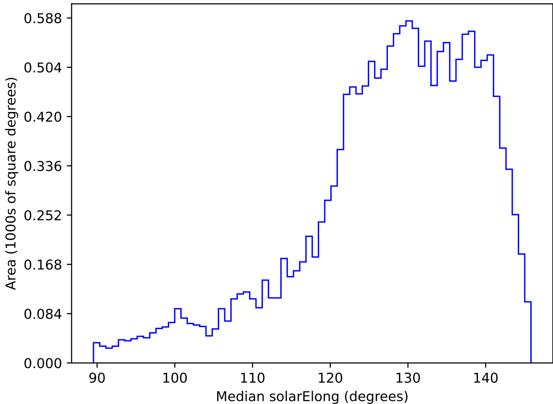
ddf_acor_sf10_lsf40_lsr10_v3.4_10yrs WFD z band: Median solarElong
