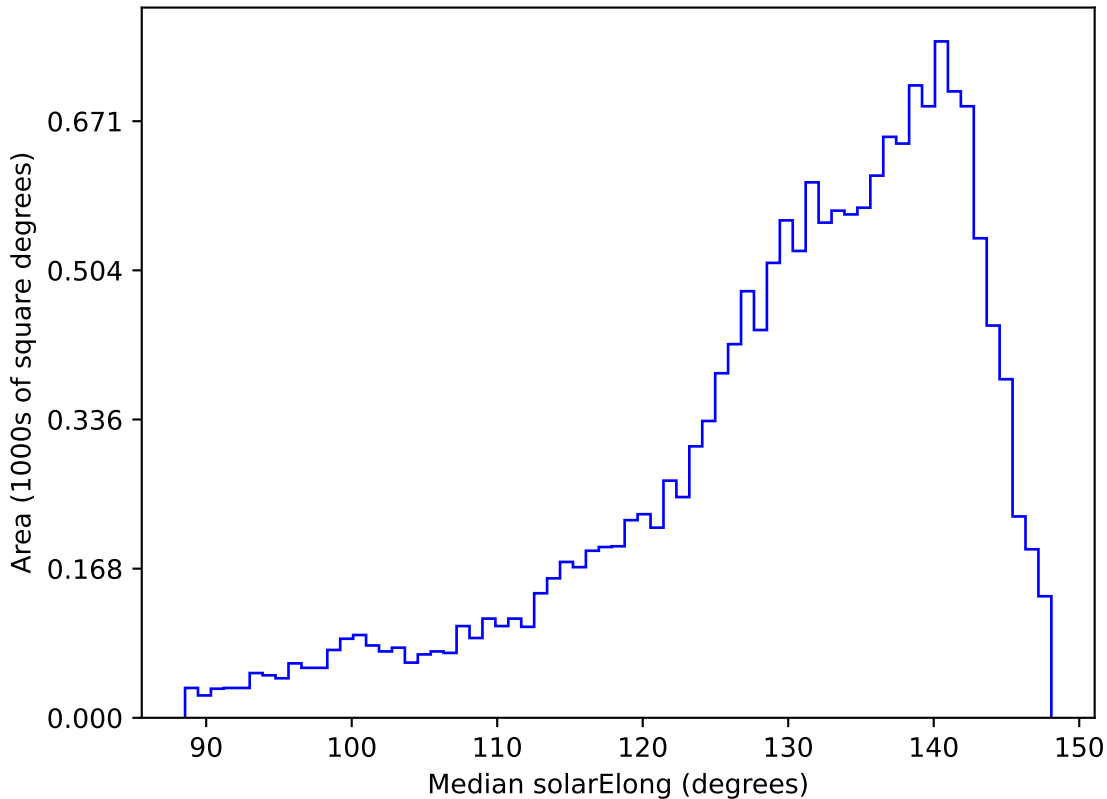
ddf_acor_sf10_lsf40_lsr10_v3.4_10yrs WFD y band: Median solarElong
