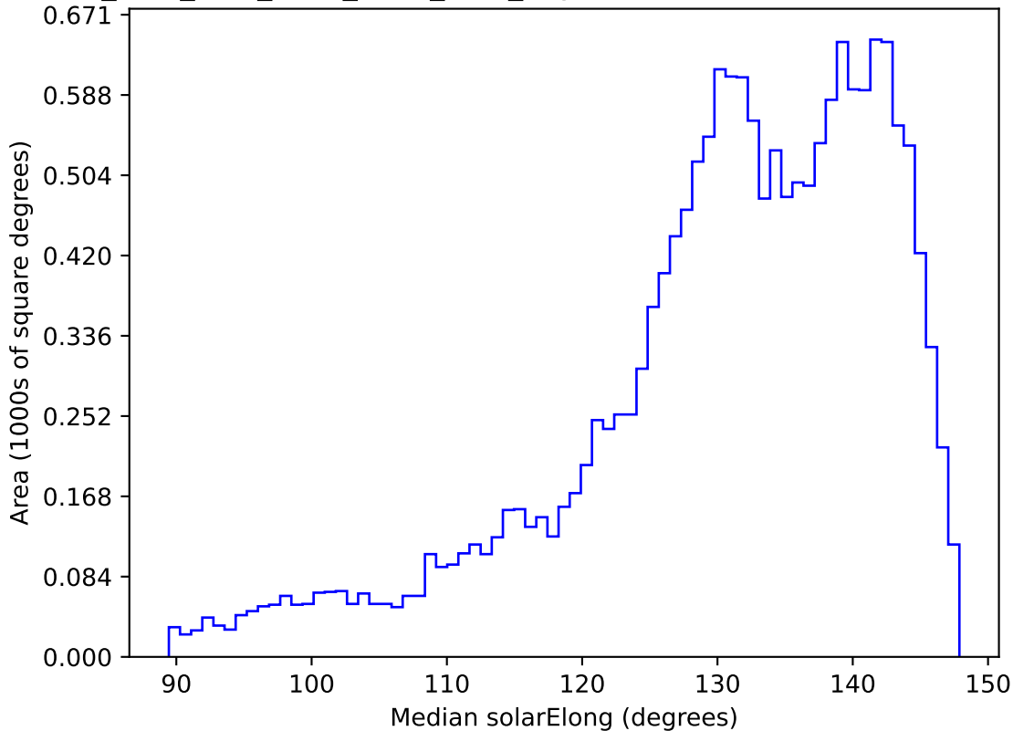
ddf_acor_sf10_lsf40_lsr10_v3.4_10yrs WFD r band: Median solarElong
