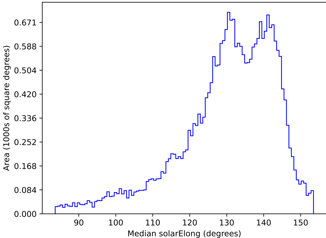
ddf_acor_sf10_lsf40_lsr10_v3.4_10yrs All sky r band: Median solarElong
