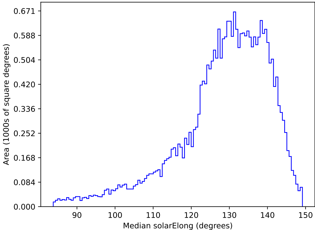
ddf_acor_sf10_lsf40_lsr10_v3.4_10yrs All sky i band: Median solarElong
