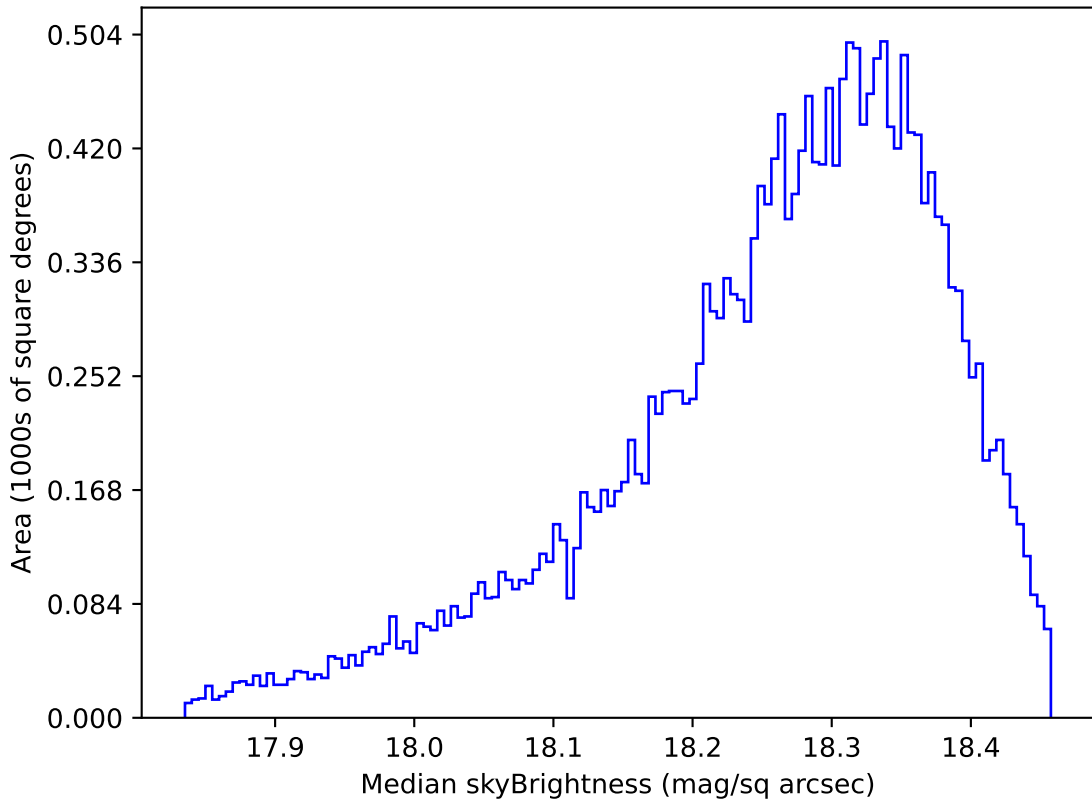
ddf_acor_sf10_lsf40_lsr10_v3.4_10yrs Yr 1 y band: Median skyBrightness
