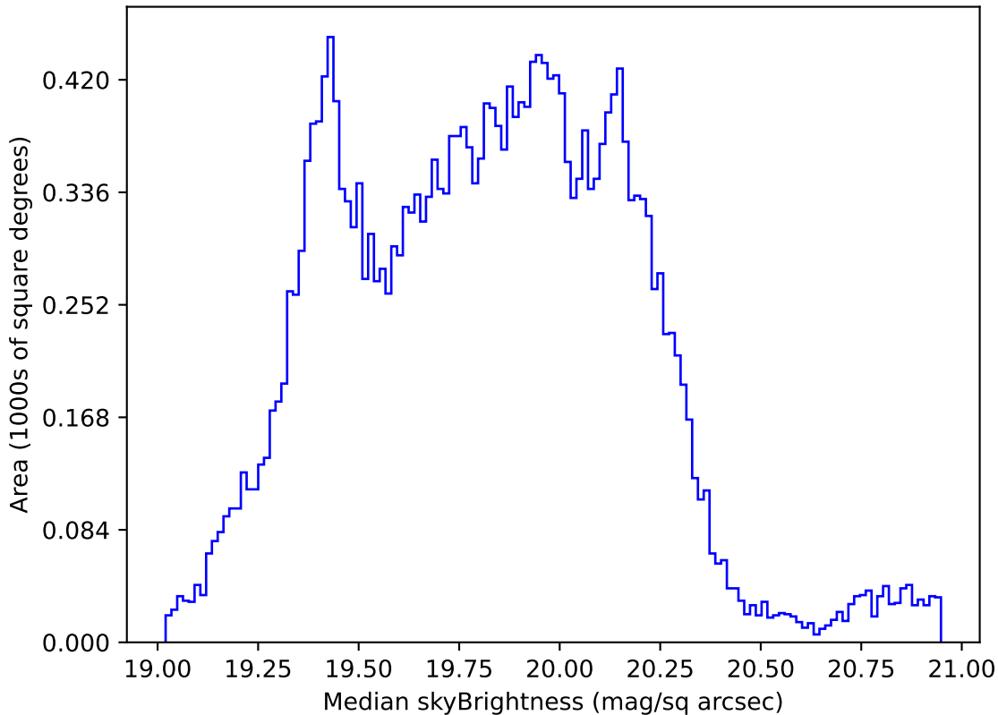
ddf_acor_sf10_lsf40_lsr10_v3.4_10yrs Yr 1 all bands: Median skyBrightness
