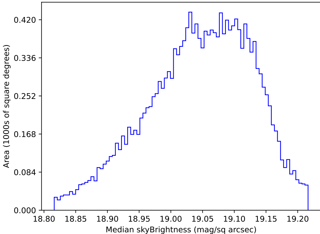
ddf_acor_sf10_lsf40_lsr10_v3.4_10yrs WFD z band: Median skyBrightness
