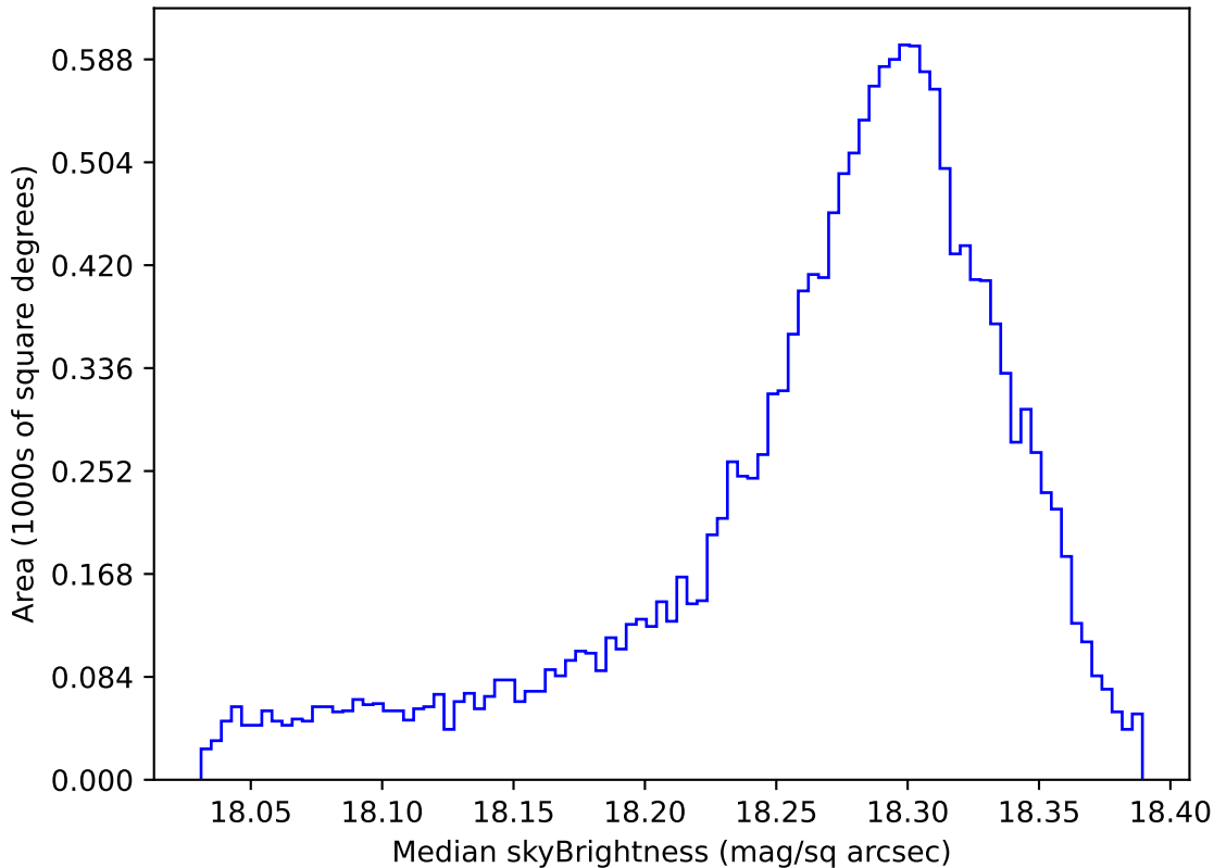
ddf_acor_sf10_lsf40_lsr10_v3.4_10yrs WFD y band: Median skyBrightness
