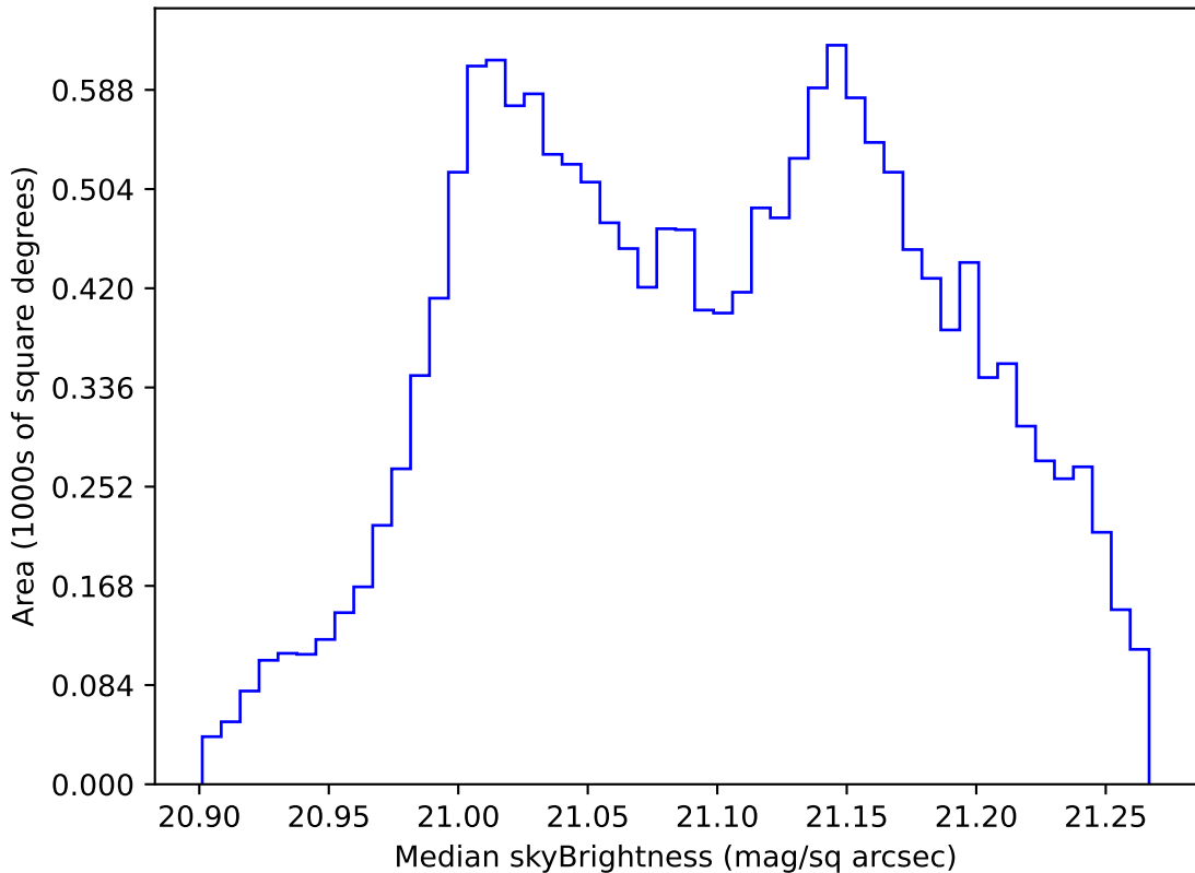
ddf_acor_sf10_lsf40_lsr10_v3.4_10yrs WFD r band: Median skyBrightness
