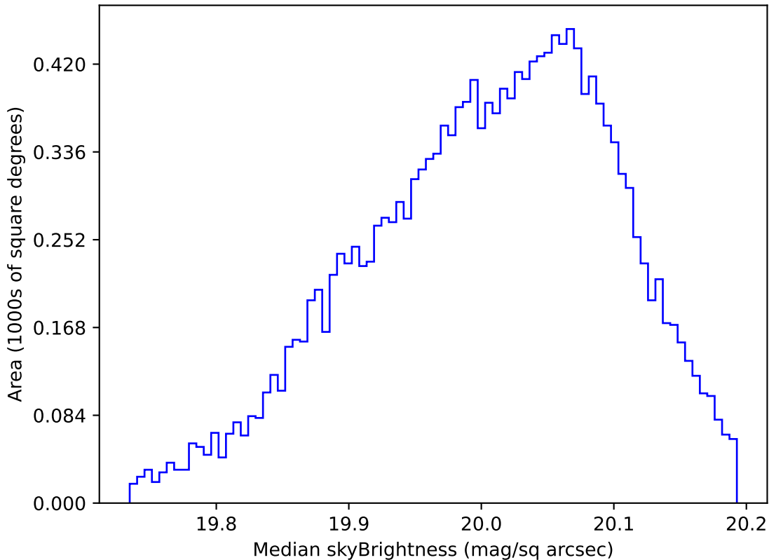
ddf_acor_sf10_lsf40_lsr10_v3.4_10yrs WFD i band: Median skyBrightness
