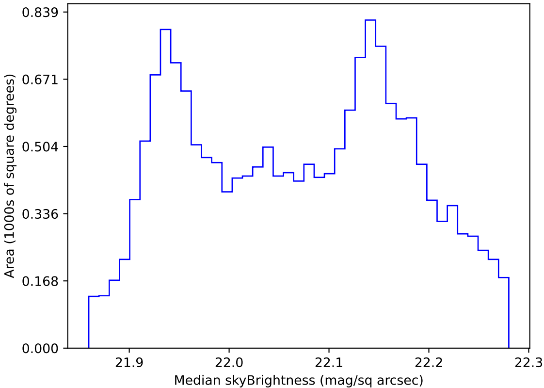
ddf_acor_sf10_lsf40_lsr10_v3.4_10yrs WFD g band: Median skyBrightness
