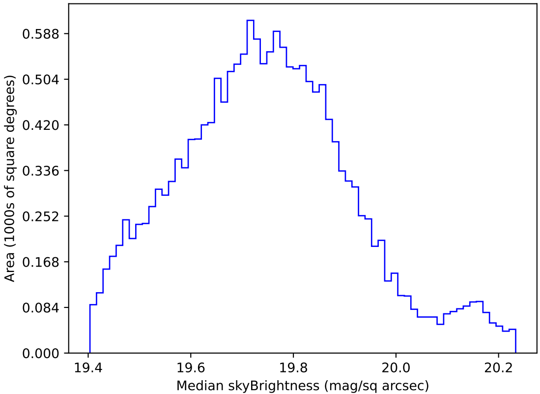
ddf_acor_sf10_lsf40_lsr10_v3.4_10yrs WFD all bands: Median skyBrightness
