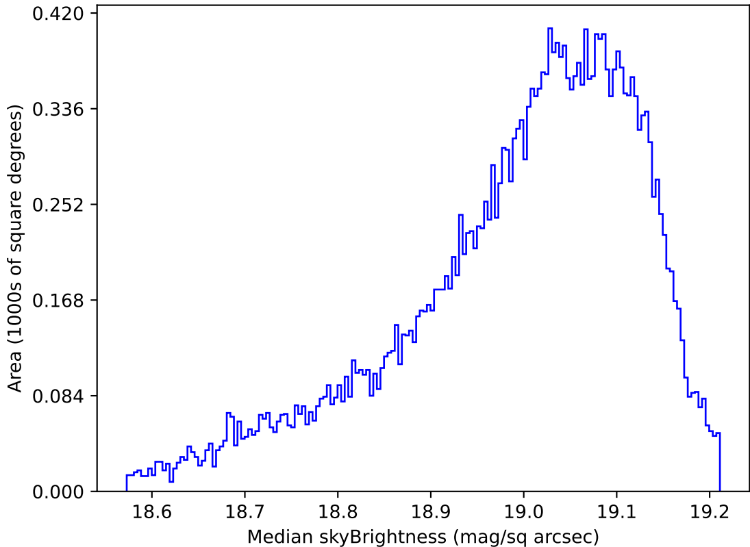
ddf_acor_sf10_lsf40_lsr10_v3.4_10yrs All sky z band: Median skyBrightness
