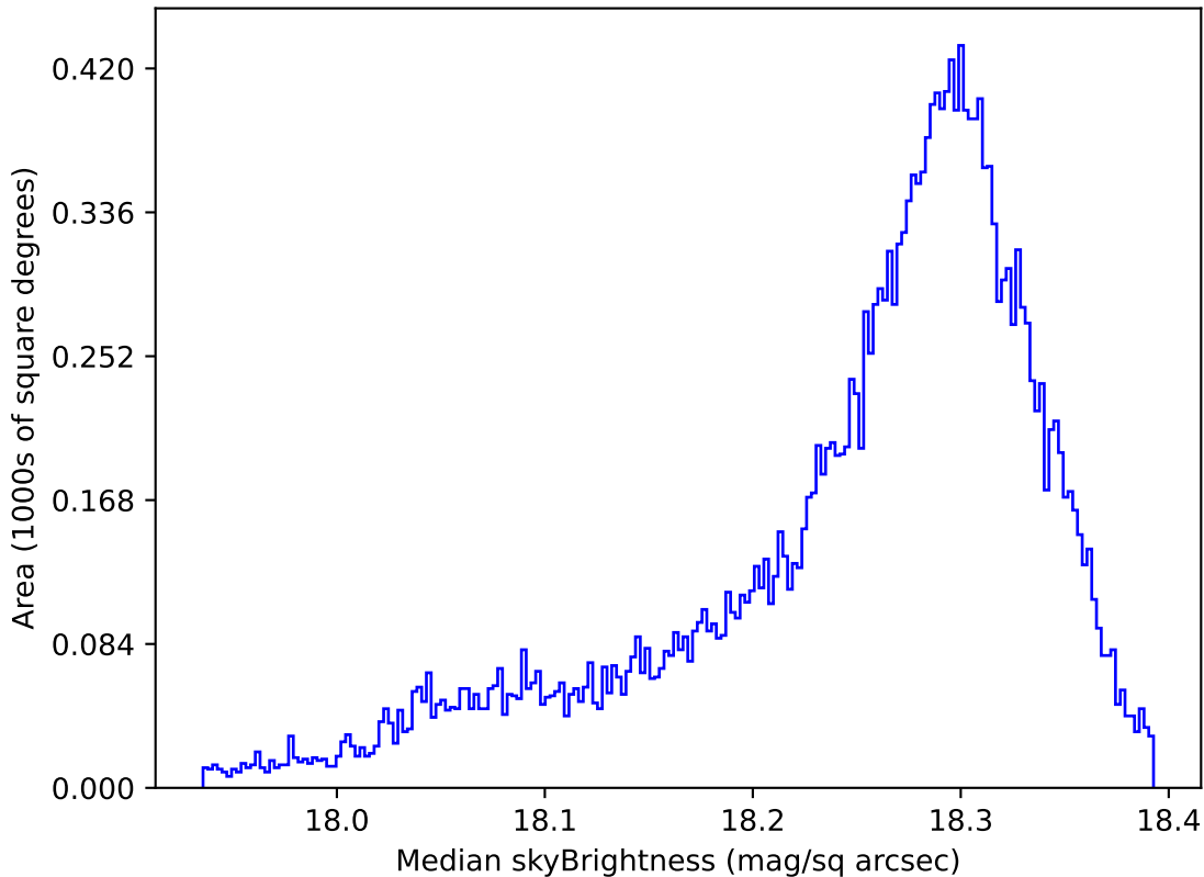
ddf_acor_sf10_lsf40_lsr10_v3.4_10yrs All sky y band: Median skyBrightness
