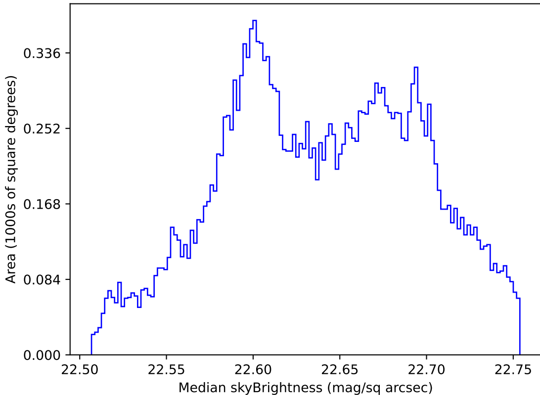
ddf_acor_sf10_lsf40_lsr10_v3.4_10yrs All sky u band: Median skyBrightness
