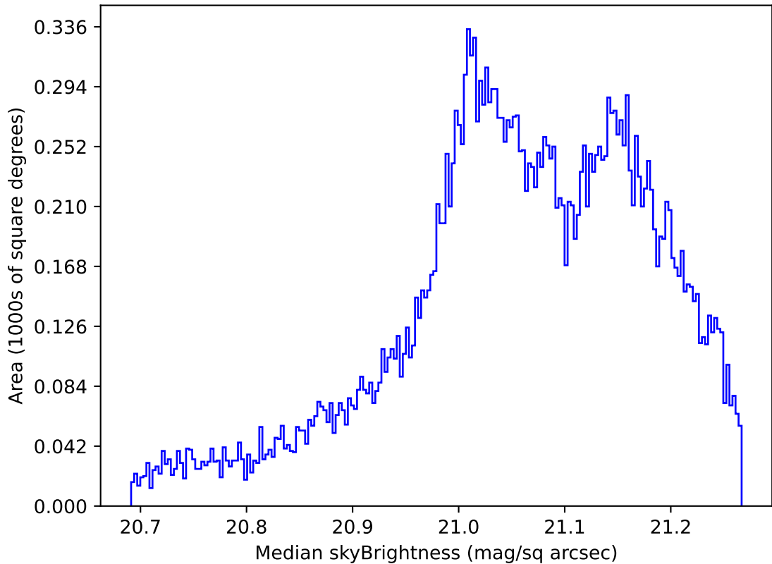
ddf_acor_sf10_lsf40_lsr10_v3.4_10yrs All sky r band: Median skyBrightness
