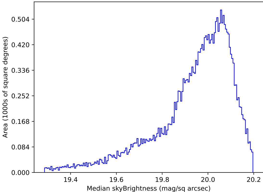
ddf_acor_sf10_lsf40_lsr10_v3.4_10yrs All sky i band: Median skyBrightness
