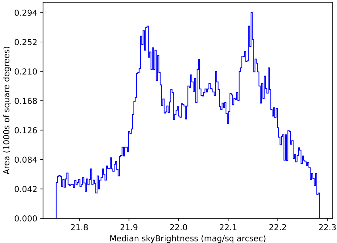
ddf_acor_sf10_lsf40_lsr10_v3.4_10yrs All sky g band: Median skyBrightness
