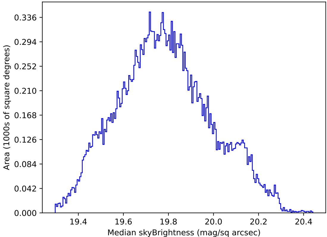
ddf_acor_sf10_lsf40_lsr10_v3.4_10yrs All sky all bands: Median skyBrightness
