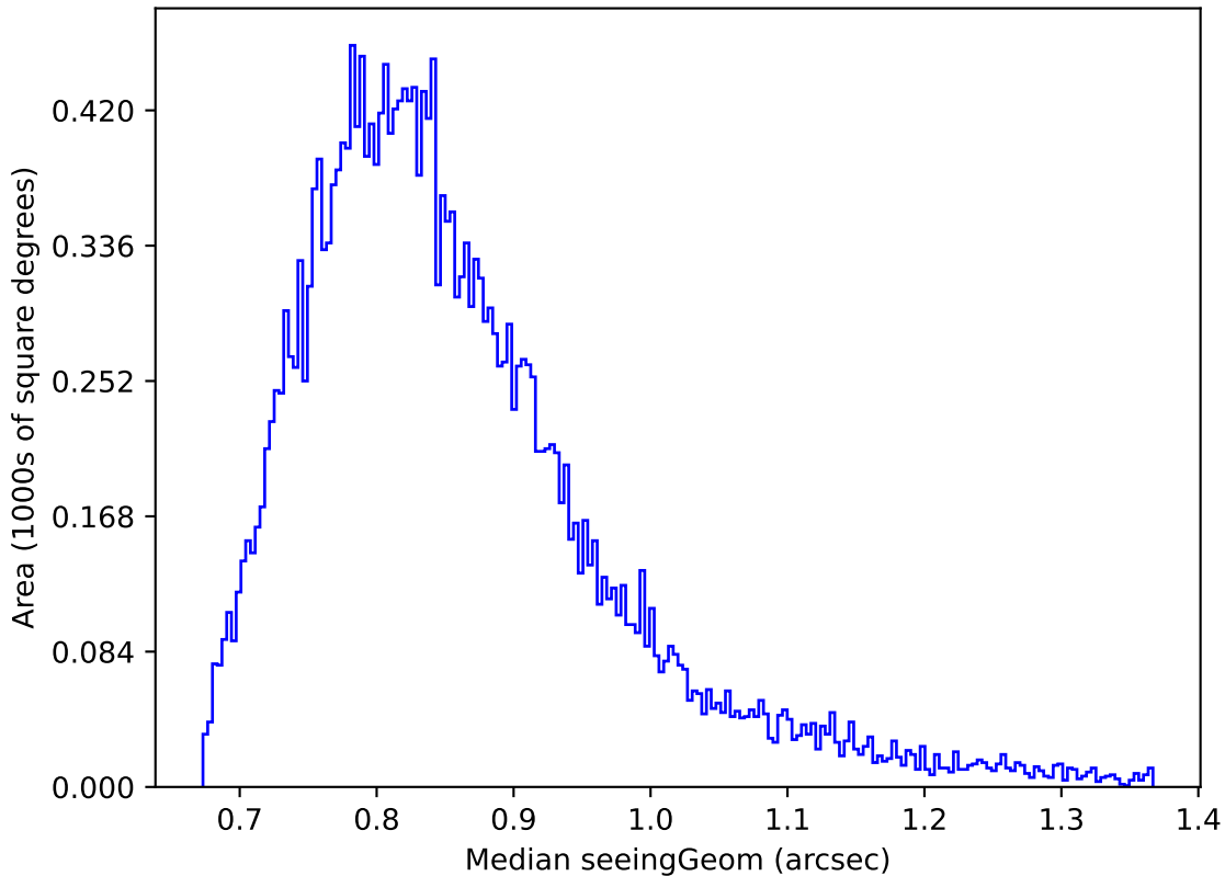
ddf_acor_sf10_lsf40_lsr10_v3.4_10yrs Yr 1 z band: Median seeingGeom
