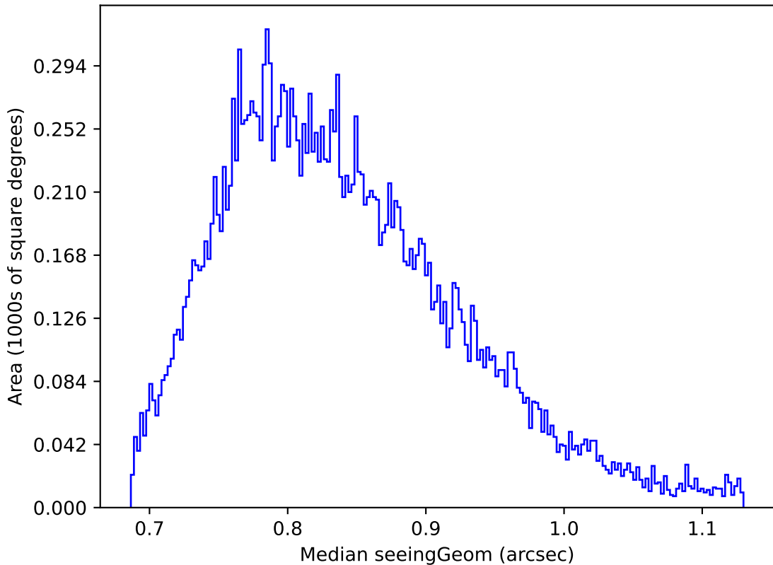
ddf_acor_sf10_lsf40_lsr10_v3.4_10yrs Yr 1 y band: Median seeingGeom
