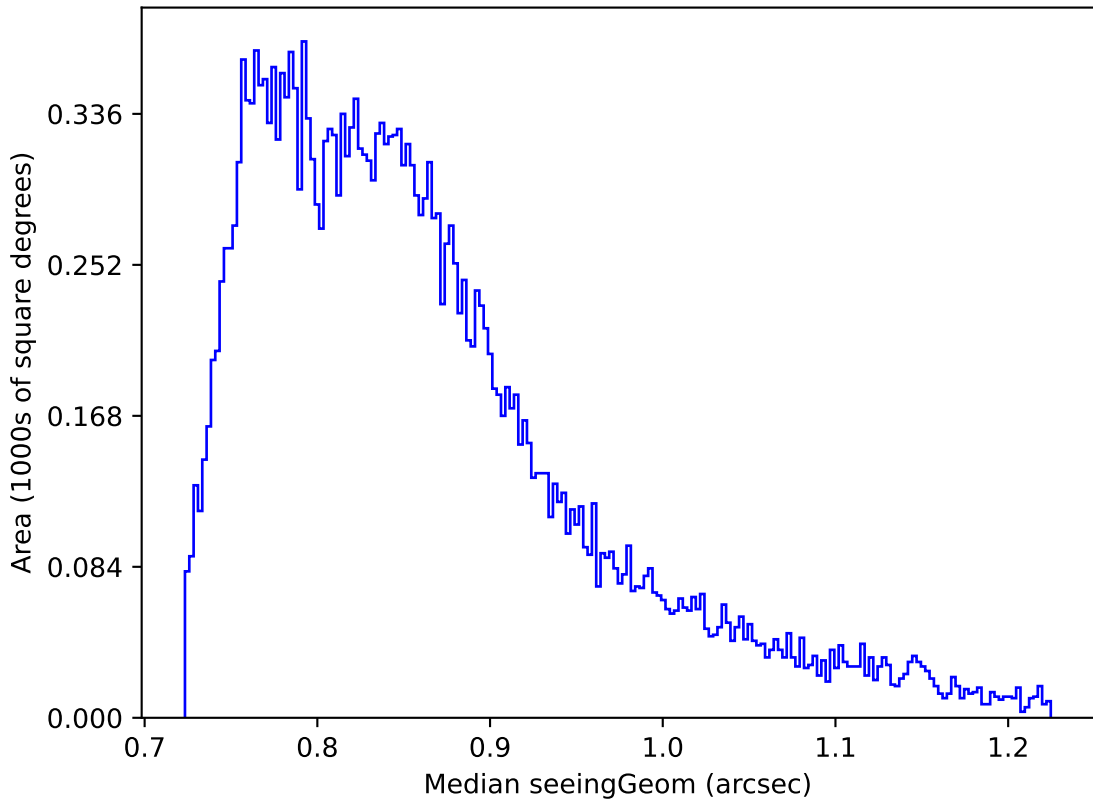
ddf_acor_sf10_lsf40_lsr10_v3.4_10yrs Yr 1 all bands: Median seeingGeom
