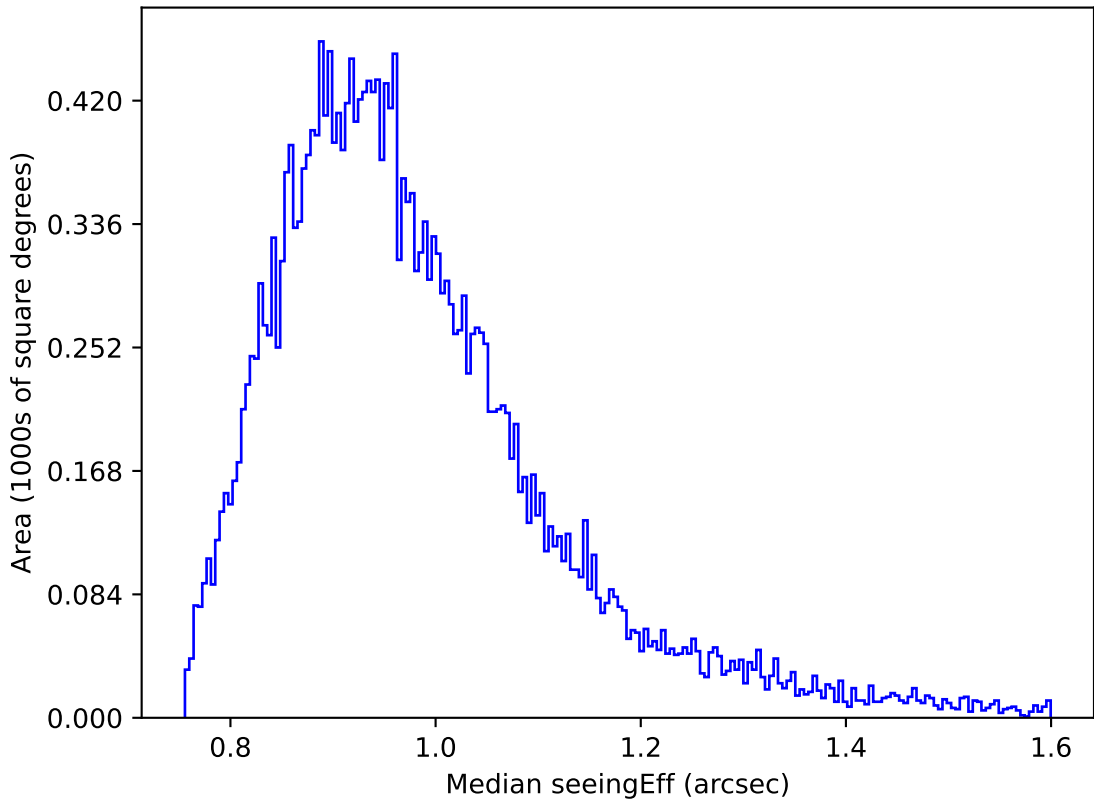
ddf_acor_sf10_lsf40_lsr10_v3.4_10yrs Yr 1 z band: Median seeingEff
