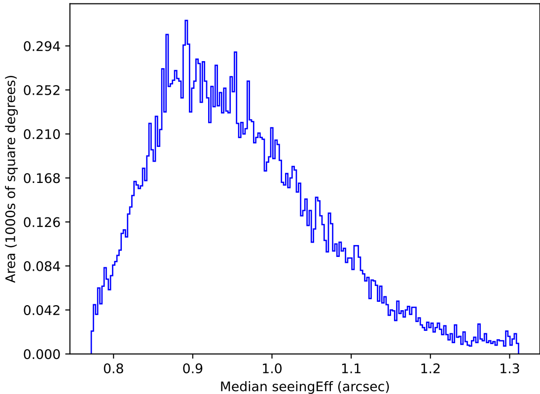
ddf_acor_sf10_lsf40_lsr10_v3.4_10yrs Yr 1 y band: Median seeingEff
