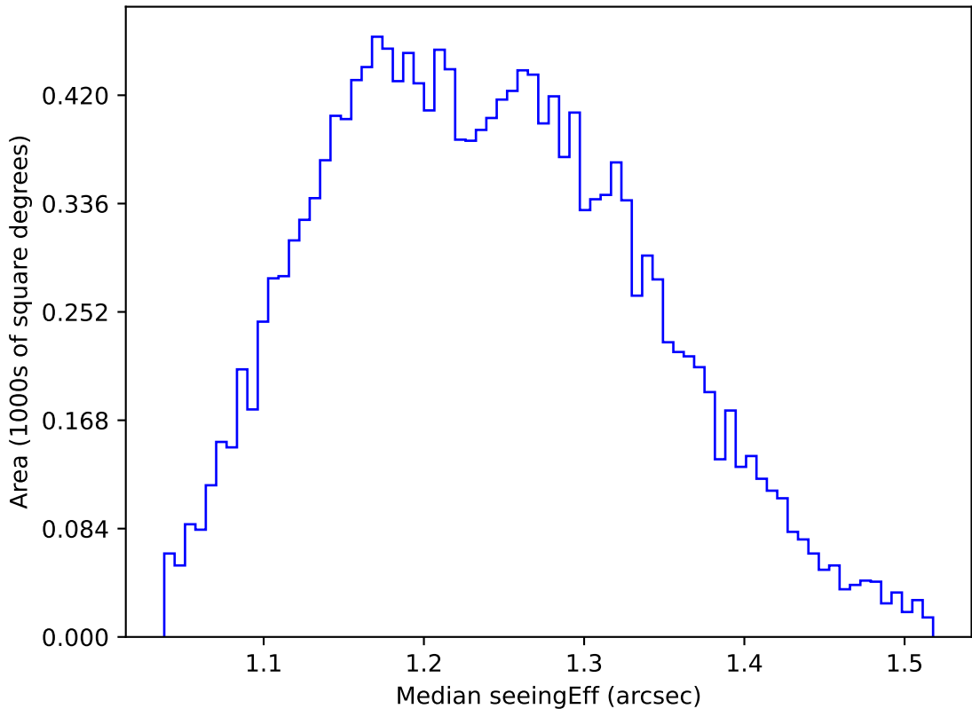
ddf_acor_sf10_lsf40_lsr10_v3.4_10yrs WFD u band: Median seeingEff
