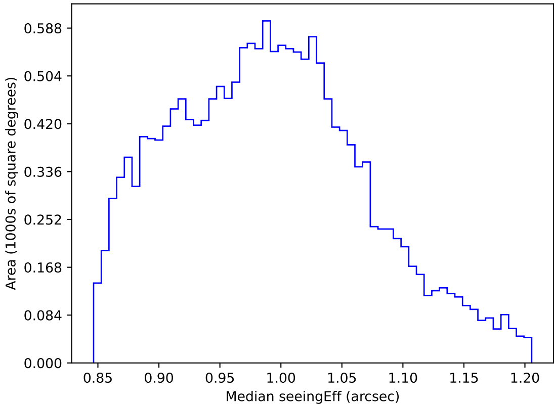
ddf_acor_sf10_lsf40_lsr10_v3.4_10yrs WFD i band: Median seeingEff
