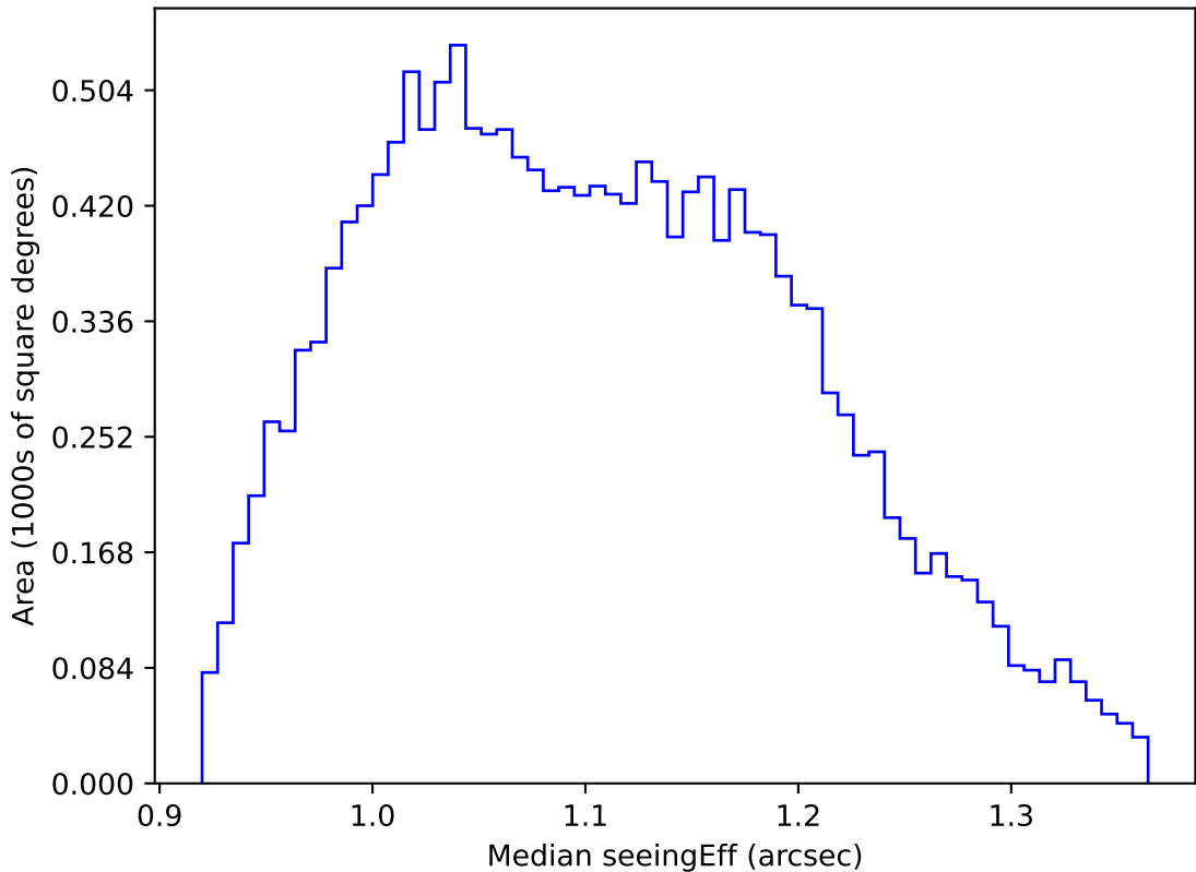
ddf_acor_sf10_lsf40_lsr10_v3.4_10yrs WFD g band: Median seeingEff
