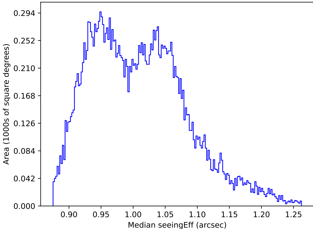
ddf_acor_sf10_lsf40_lsr10_v3.4_10yrs All sky y band: Median seeingEff
