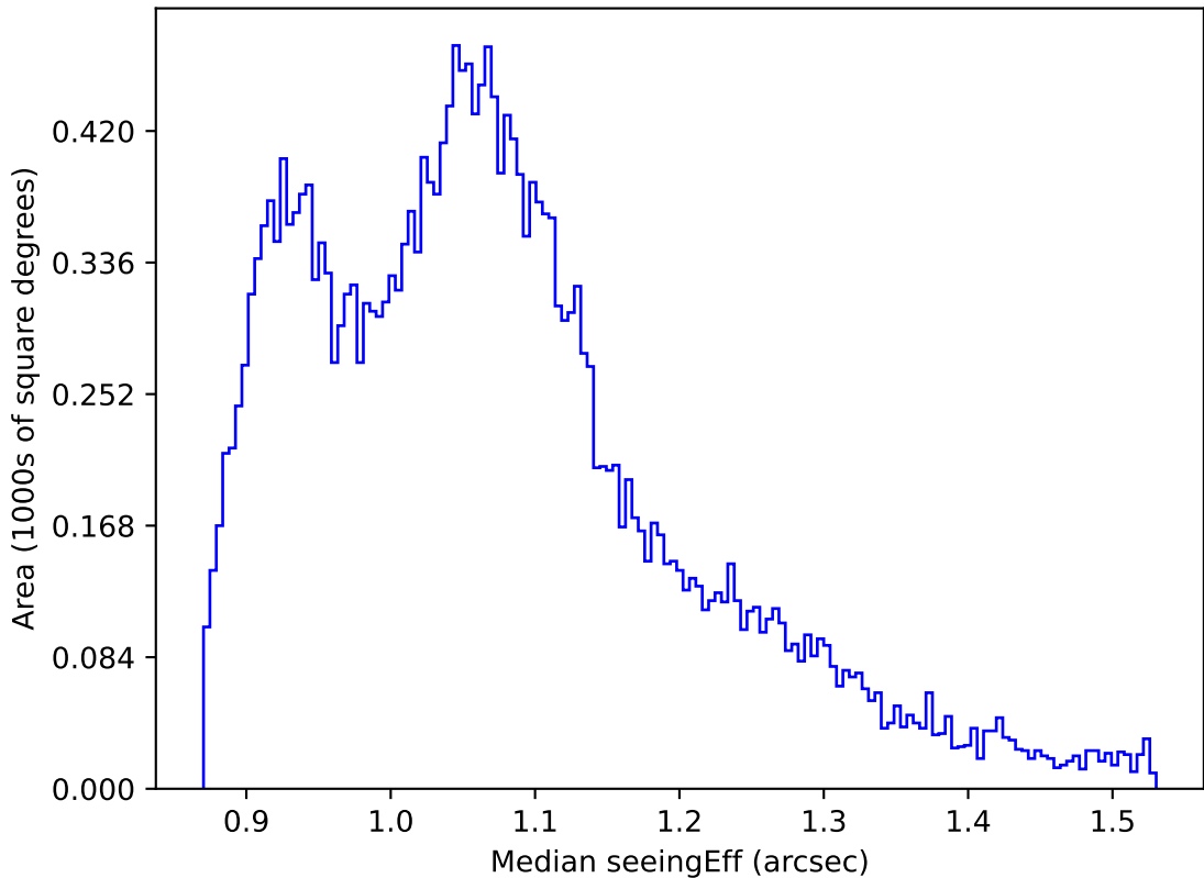
ddf_acor_sf10_lsf40_lsr10_v3.4_10yrs All sky r band: Median seeingEff
