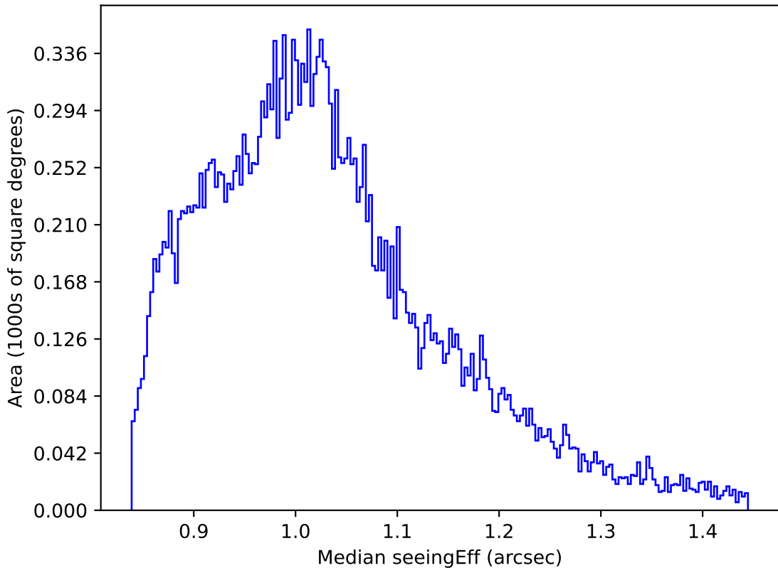
ddf_acor_sf10_lsf40_lsr10_v3.4_10yrs All sky i band: Median seeingEff
