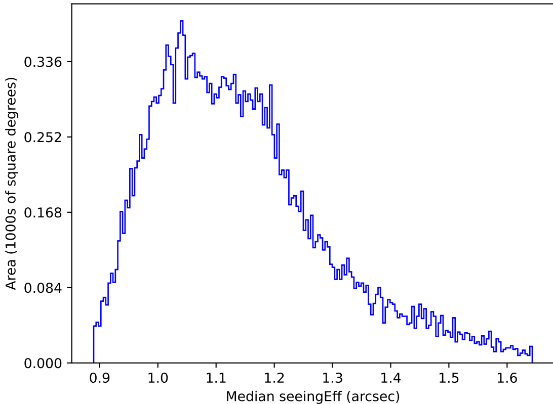
ddf_acor_sf10_lsf40_lsr10_v3.4_10yrs All sky g band: Median seeingEff
