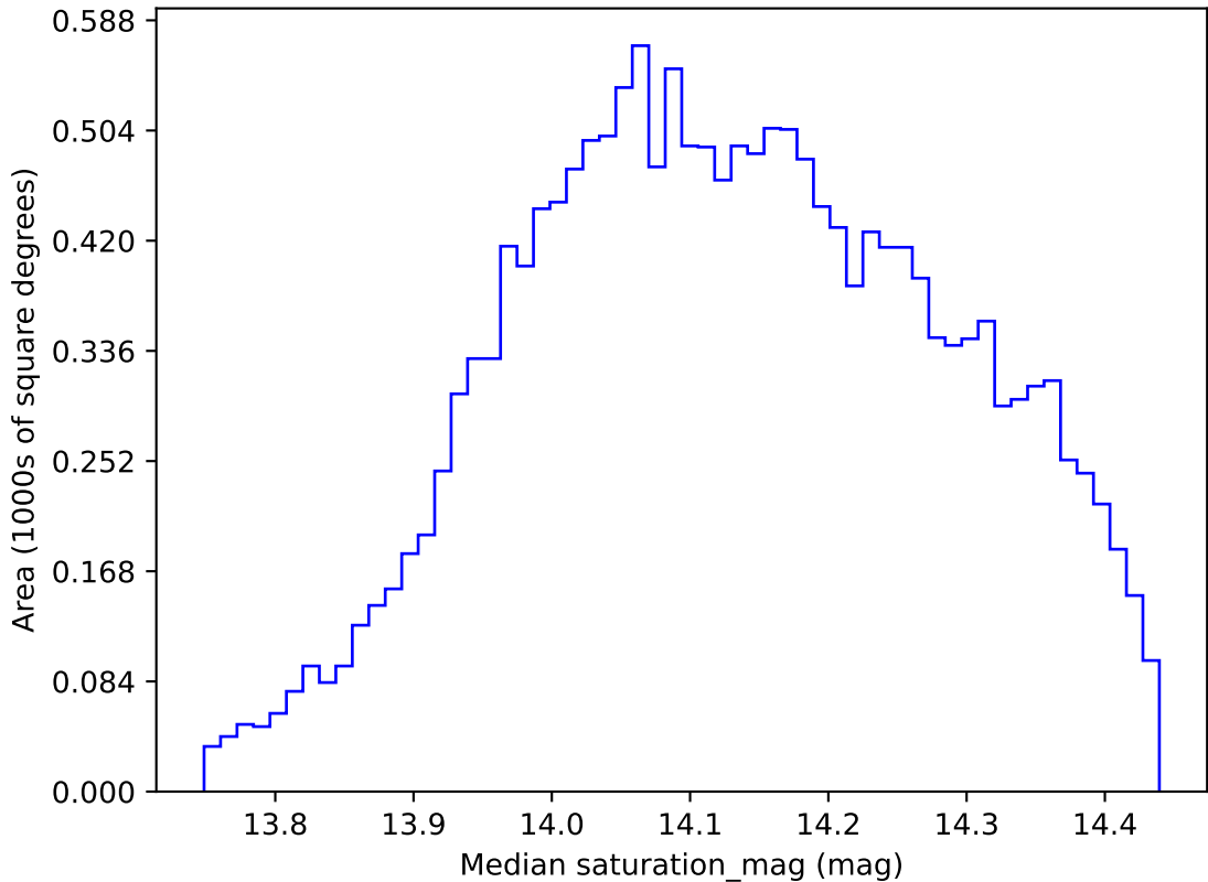
ddf_acor_sf10_lsf40_lsr10_v3.4_10yrs WFD z band: Median saturation_mag
