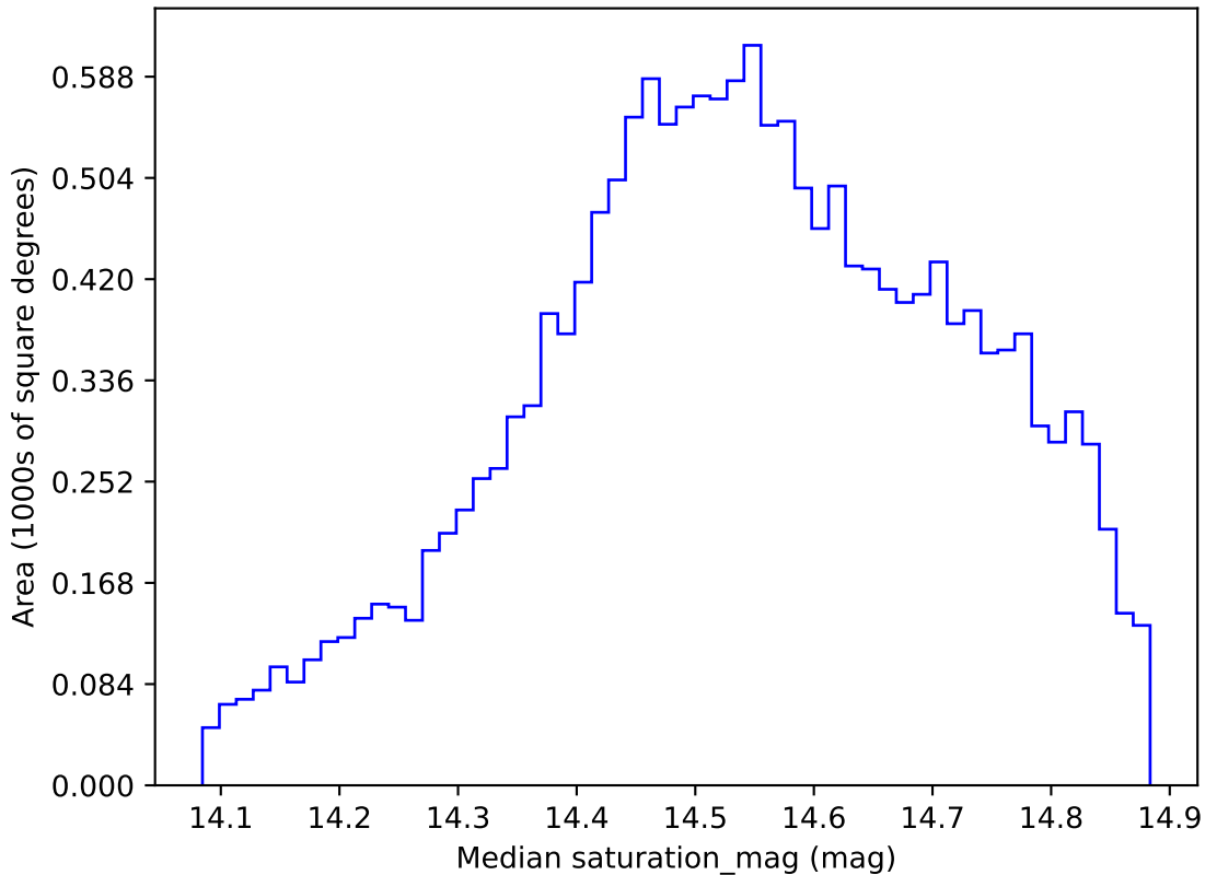
ddf_acor_sf10_lsf40_lsr10_v3.4_10yrs WFD i band: Median saturation_mag
