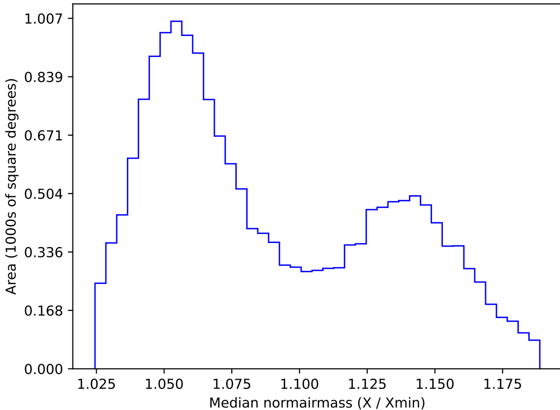
ddf_acor_sf10_lsf40_lsr10_v3.4_10yrs WFD y band: Median normairmass
