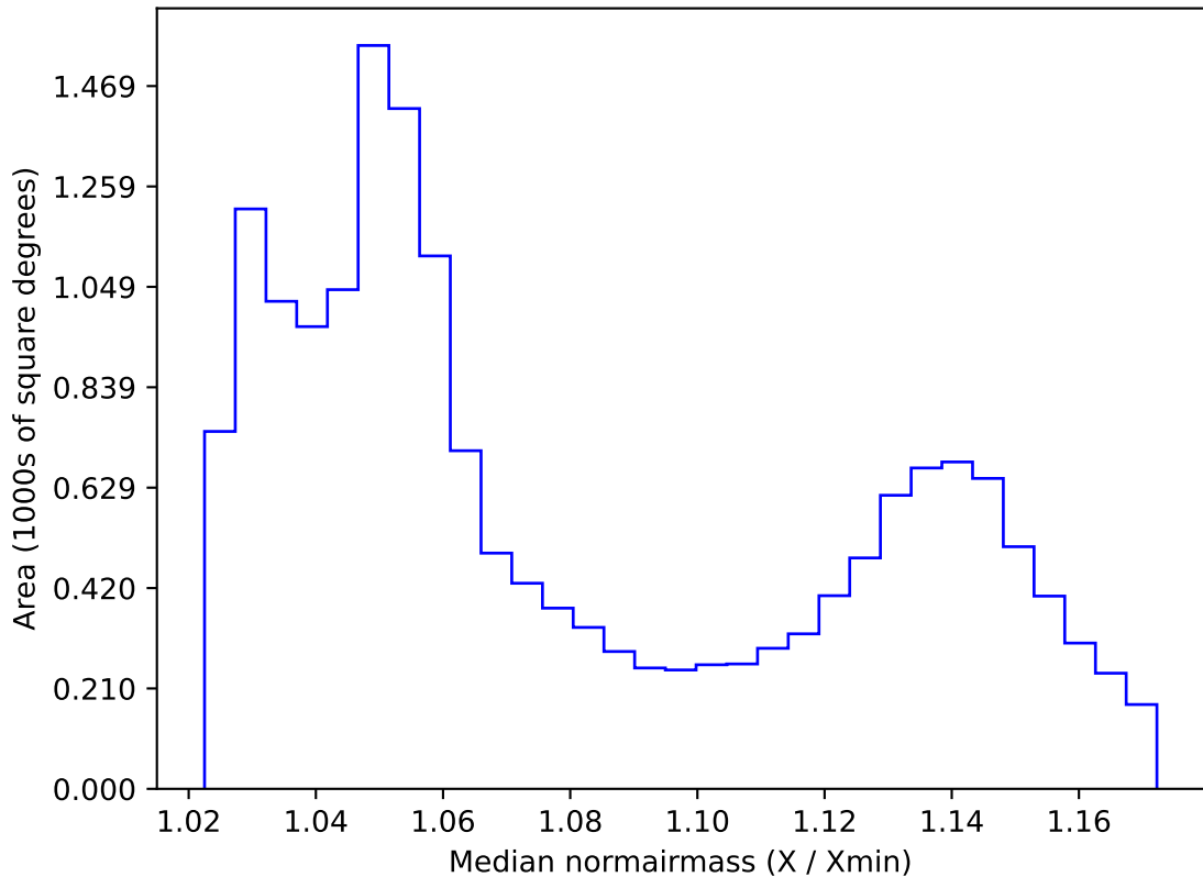
ddf_acor_sf10_lsf40_lsr10_v3.4_10yrs WFD all bands: Median normairmass
