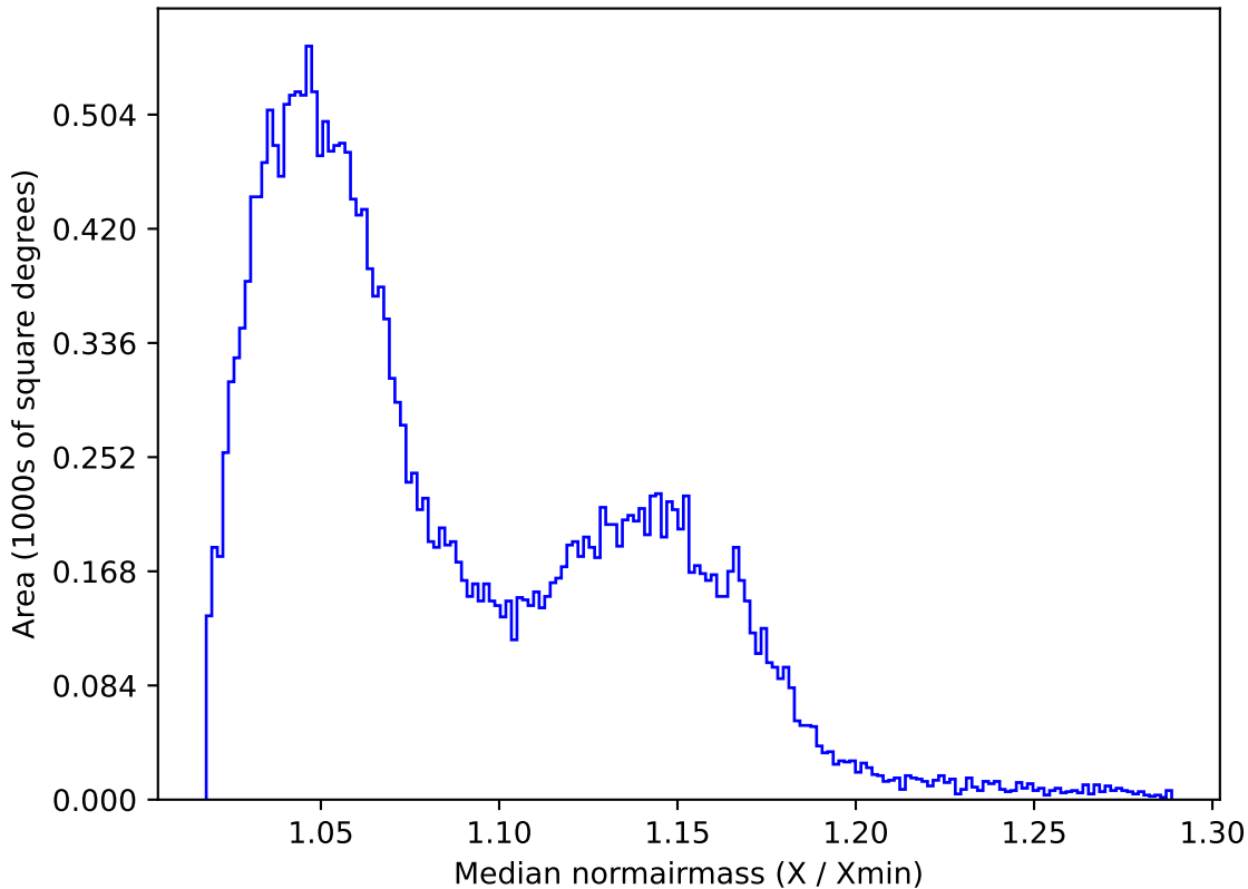
ddf_acor_sf10_lsf40_lsr10_v3.4_10yrs All sky z band: Median normairmass
