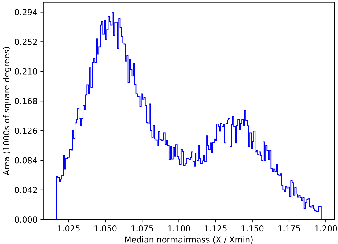
ddf_acor_sf10_ls40_lsr10_v3.4_10yrs All sky y band: Median normairmass
