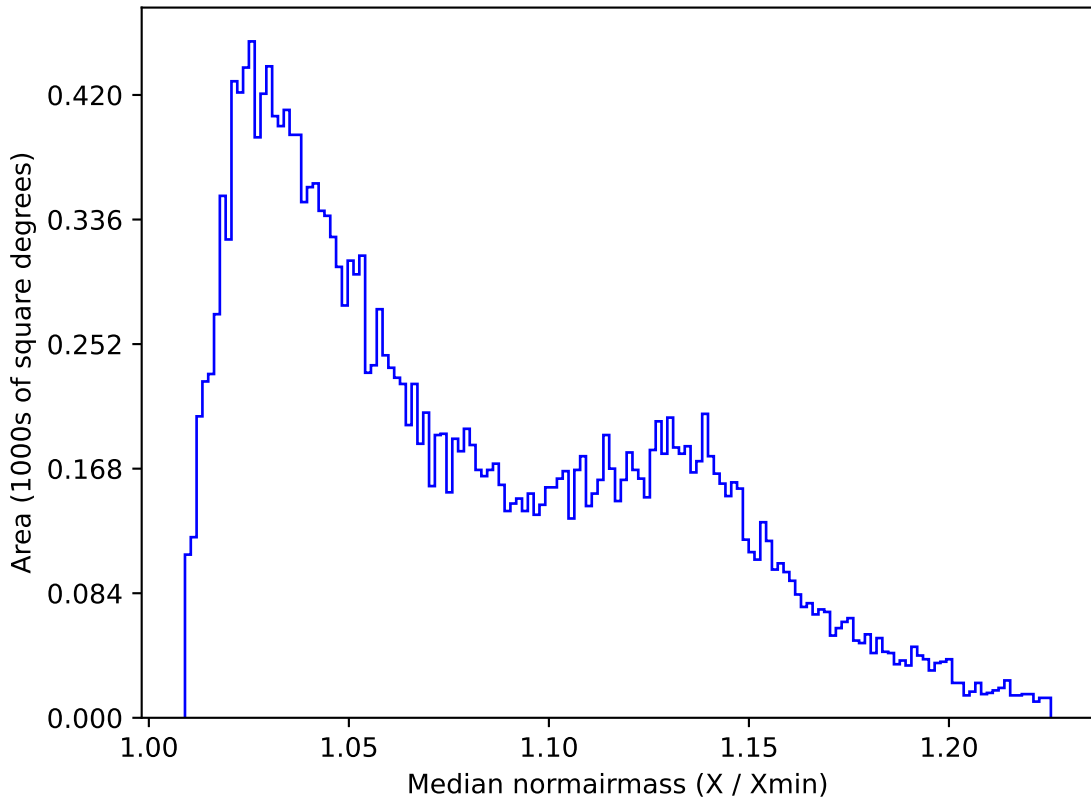
ddf_acor_sf10_ls40_lsr10_v3.4_10yrs All sky u band: Median normairmass
