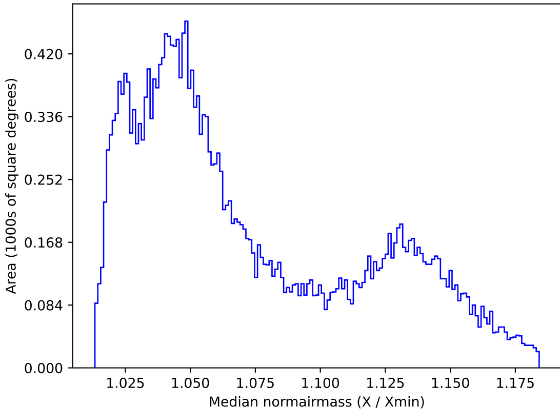
ddf_acor_sf10_ls40_lsr10_v3.4_10yrs All sky r band: Median normairmass
